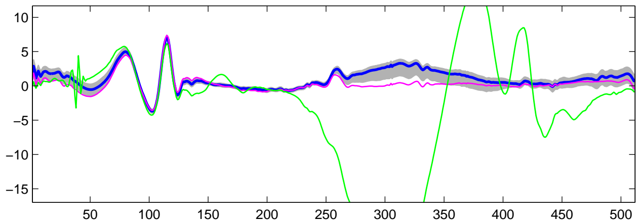
Estimated U_4(t) using R-WFMM: t_1 data, run 3
