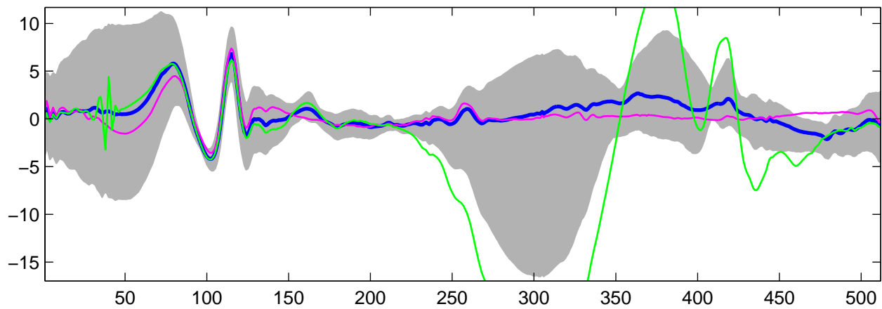
Estimated U_4(t) using G-WFMM: t_1 data, run 3
