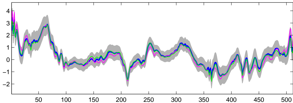
Estimated U_4(t) using G-WFMM: t_3 data, run 3
