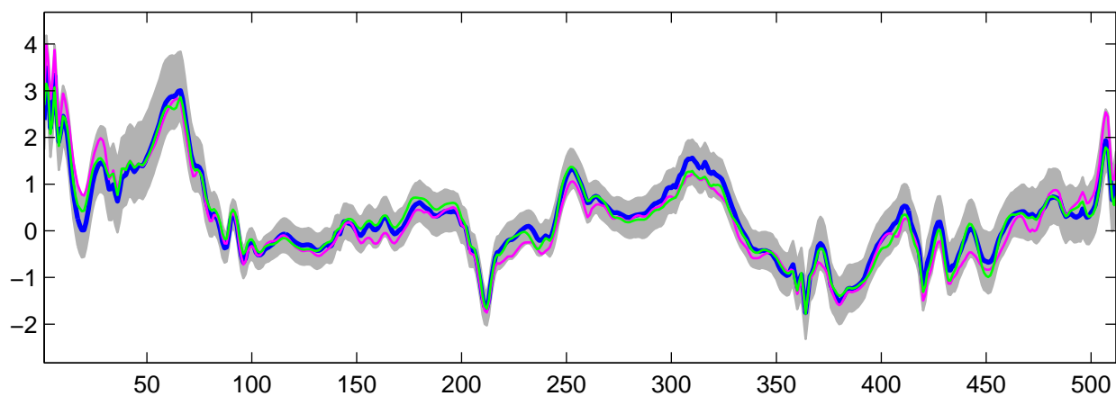
Estimated U_4(t) using R-WFMM: t_3 data, run 3
