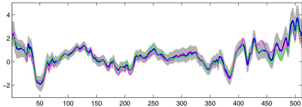
Estimated U_5(t) using R-WFMM: DE data, run 3
