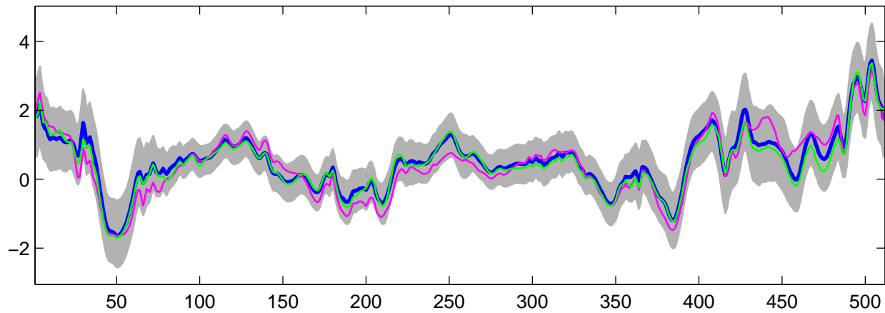
Estimated U_5(t) using G-WFMM: DE data, run 3
