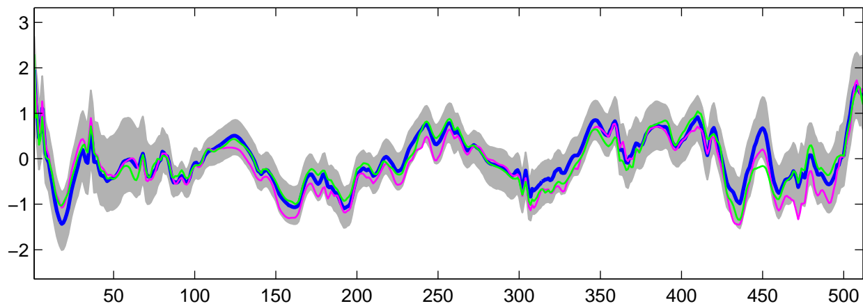
Estimated U_5(t) using R-WFMM: t_3 data, run 3
