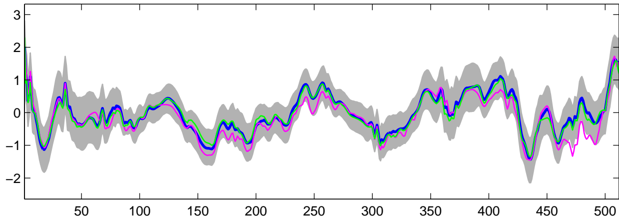
Estimated U_5(t) using G-WFMM: t_3 data, run 3
