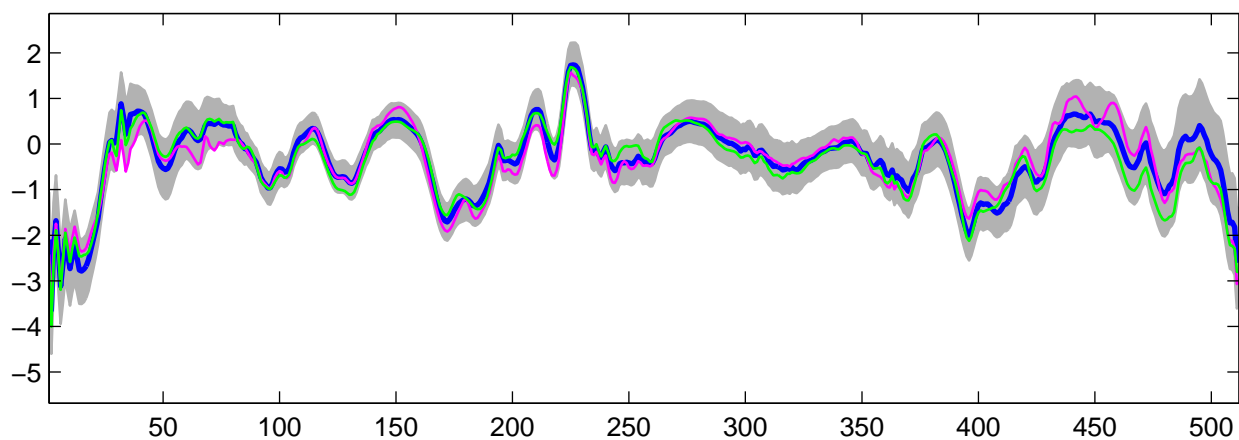
Estimated U_6(t) using R-WFMM: DE data, run 3
