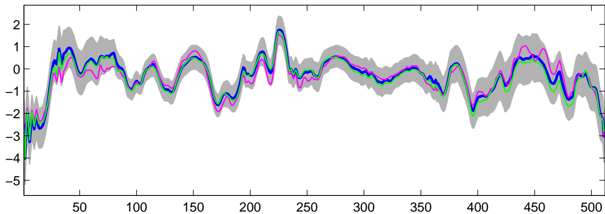
Estimated U_6(t) using G-WFMM: DE data, run 3
