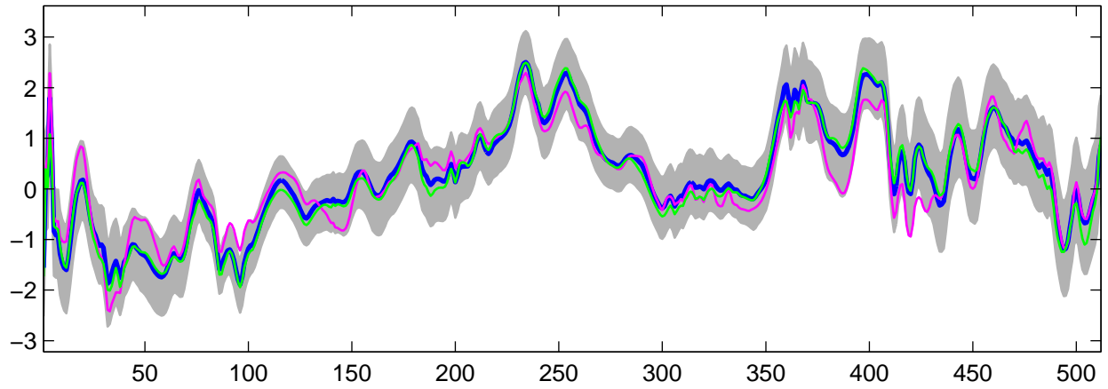
Estimated U_6(t) using G-WFMM: Normal data, run 3
