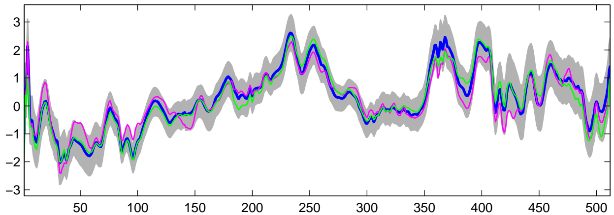
Estimated U_6(t) using R-WFMM: Normal data, run 3
