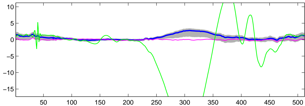
Estimated U_{\hat{\theta}}(t) using R-WFMM: t_1 data, run 3
