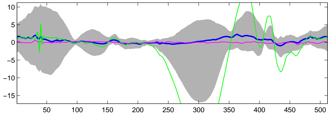
Estimated U_{\hat{\theta}}(t) using G-WFMM: t_1 data, run 3
