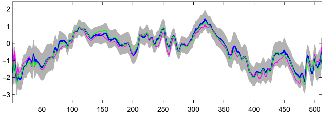
Estimated U_6(t) using G-WFMM: t_3 data, run 3
