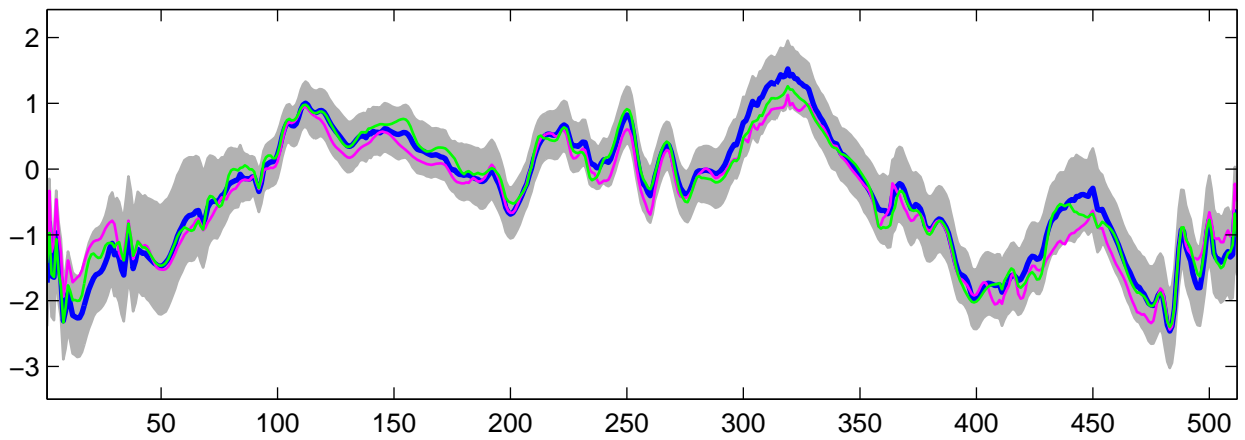
Estimated U_6(t) using R-WFMM: t_3 data, run 3
