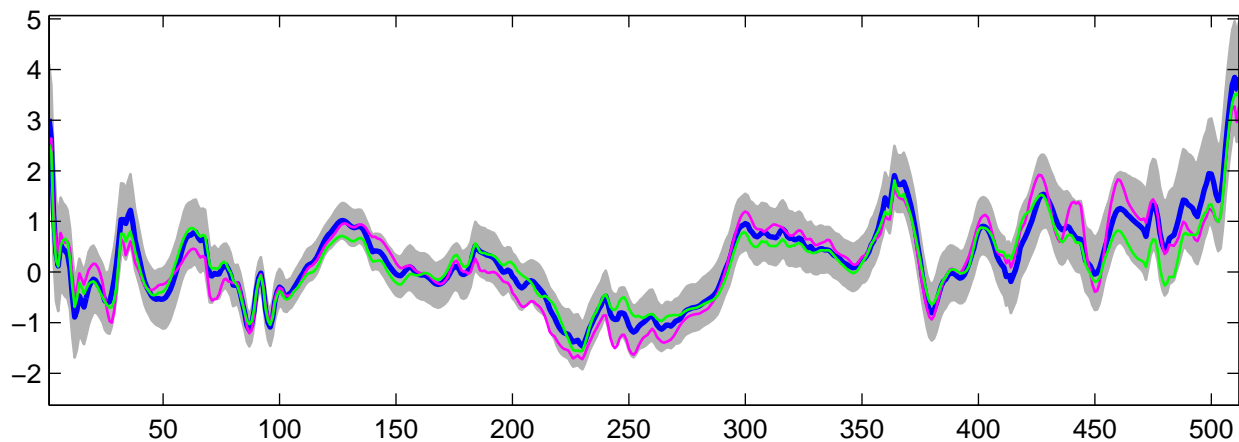
Estimated U_7(t) using R-WFMM: DE data, run 3
