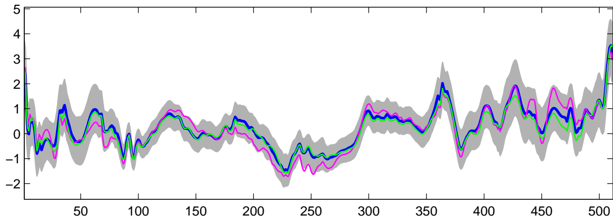
Estimated U_7(t) using G-WFMM: DE data, run 3
