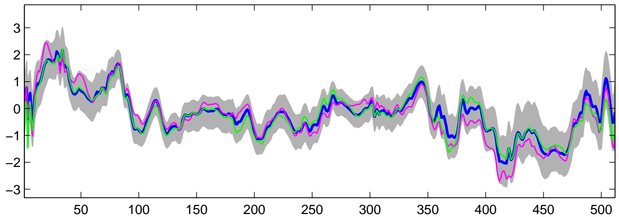
Estimated U_7(t) using R-WFMM: Normal data, run 3
