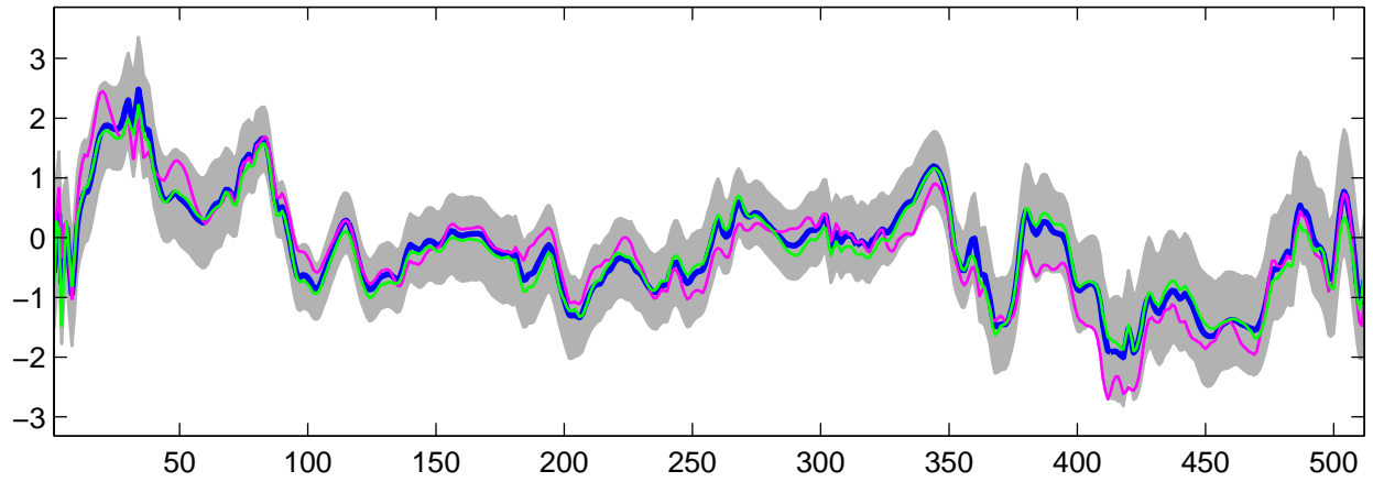
Estimated U_7(t) using G-WFMM: Normal data, run 3
