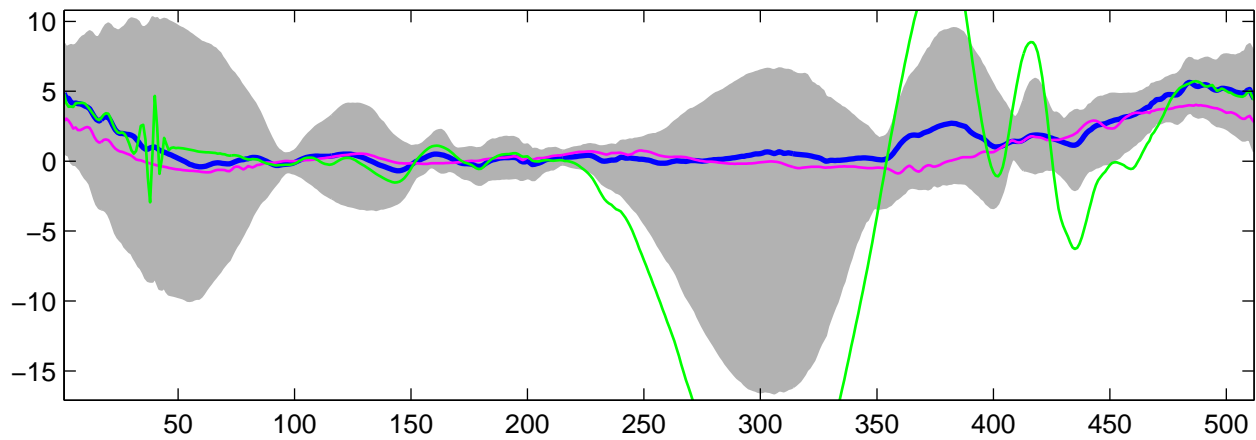
Estimated U_7(t) using G-WFMM: t_1 data, run 3
