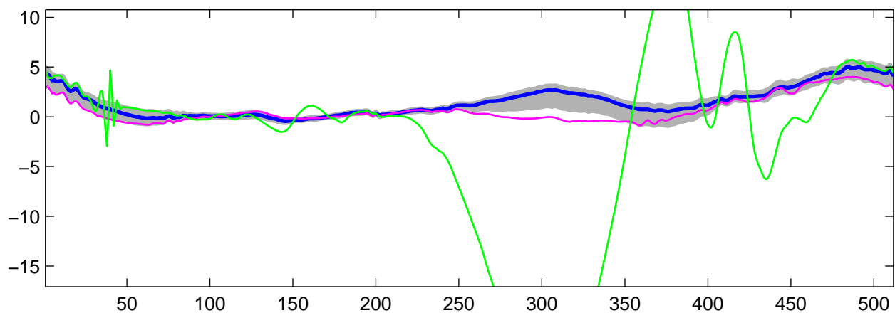
Estimated U_7(t) using R-WFMM: t_1 data, run 3
