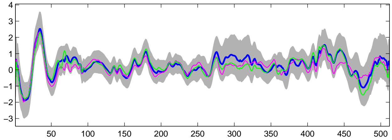
Estimated U_7(t) using G-WFMM: t_2 data, run 3
