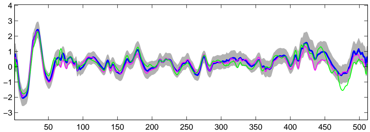
Estimated U_7(t) using R-WFMM: t_2 data, run 3
