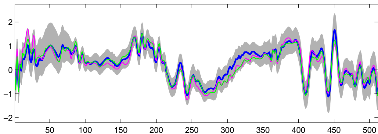
Estimated U_7(t) using R-WFMM: t_3 data, run 3
