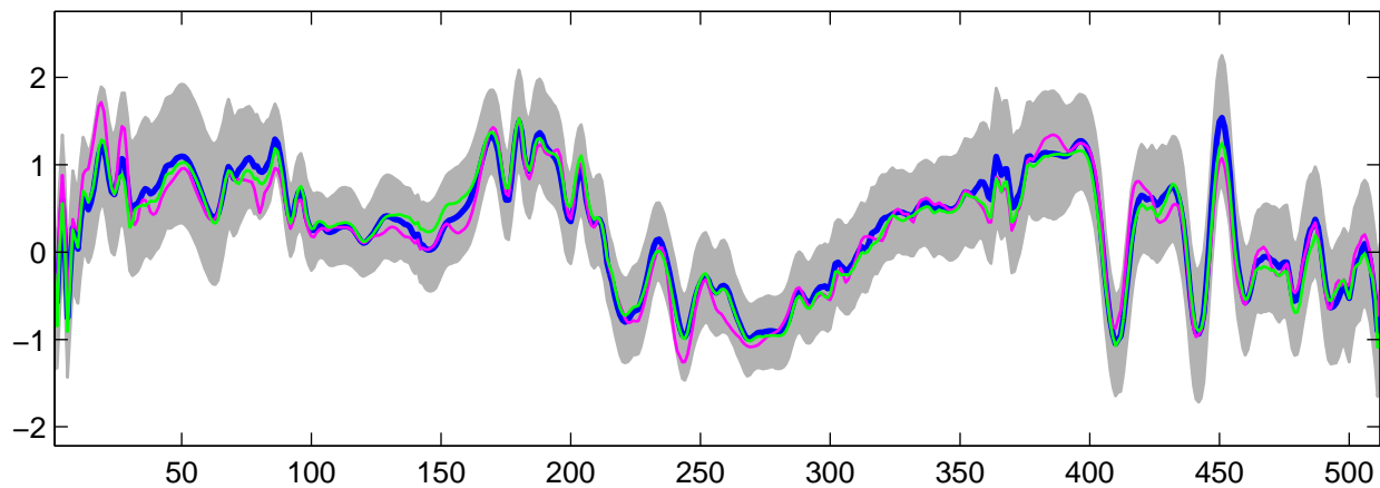
Estimated U_7(t) using G-WFMM: t_3 data, run 3
