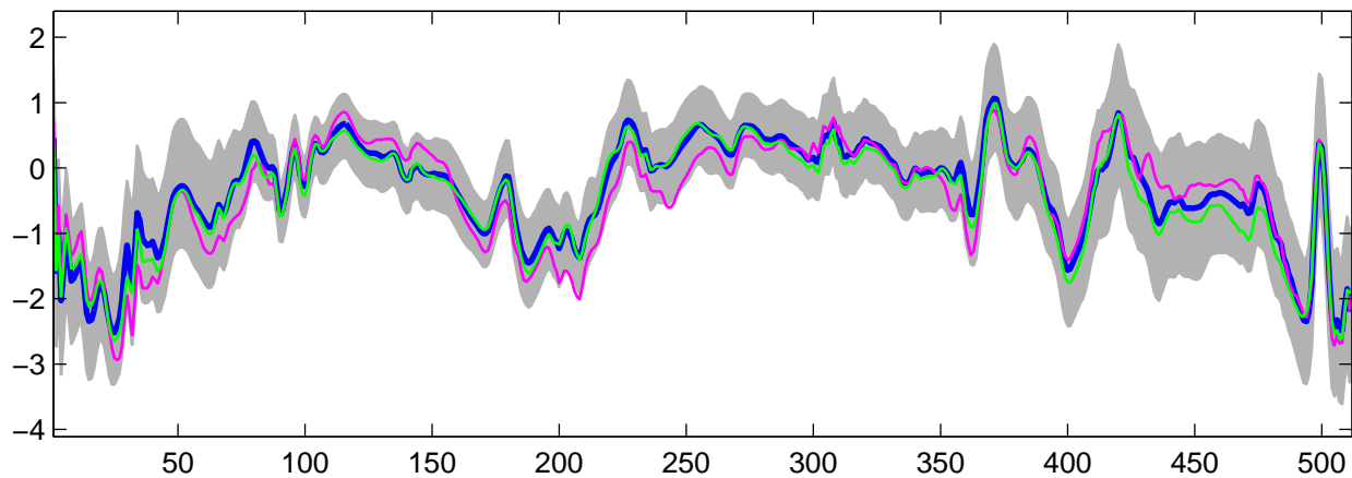
Estimated U_g(t) using G-WFMM: DE data, run 3
