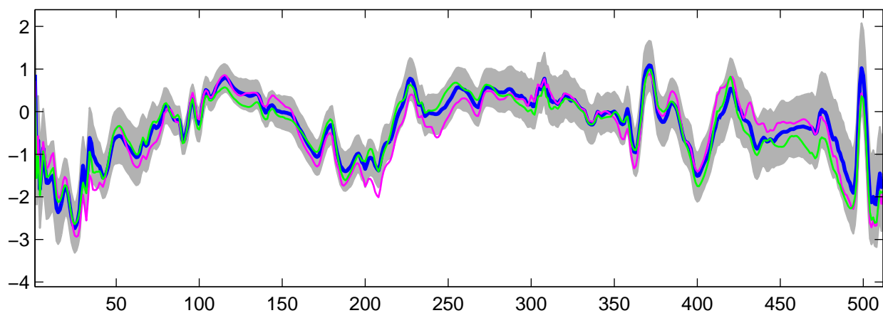
Estimated U_g(t) using R-WFMM: DE data, run 3
