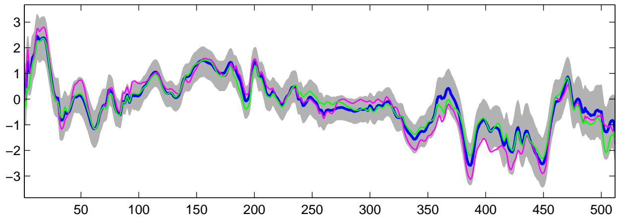
Estimated U_g(t) using R-WFMM: Normal data, run 3
