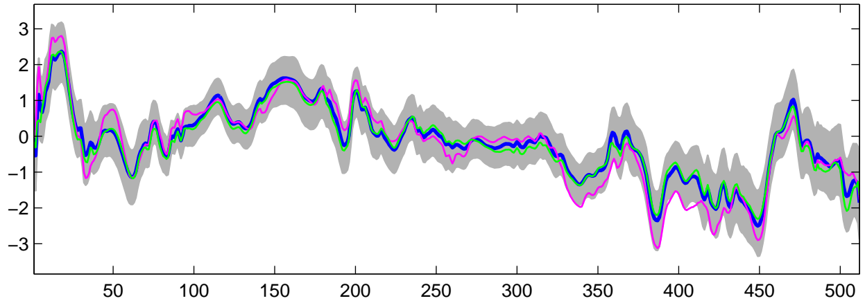
Estimated U_g(t) using G-WFMM: Normal data, run 3
