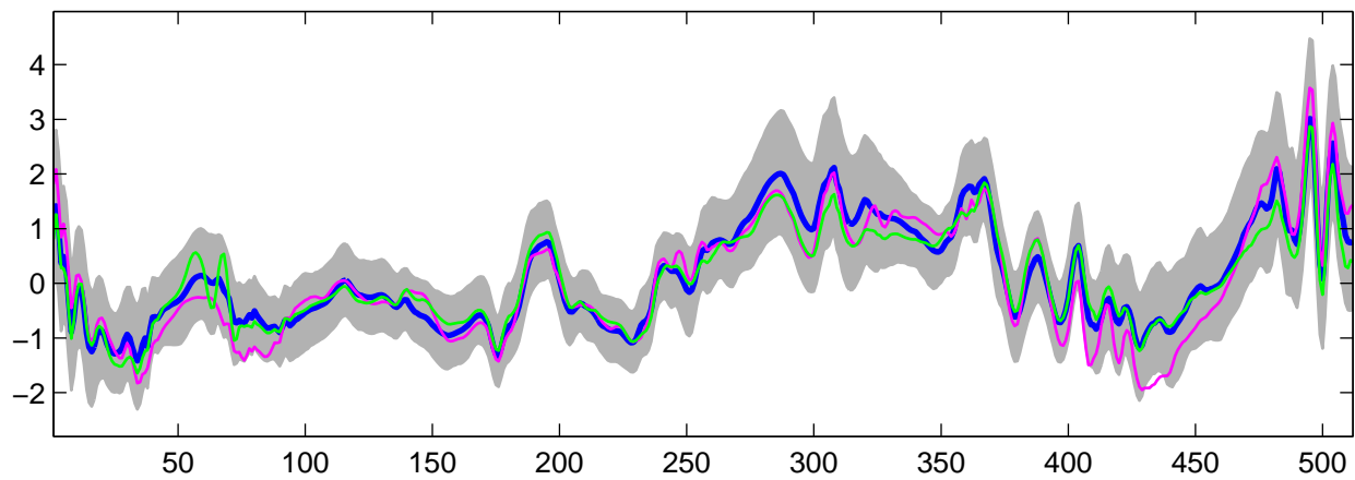
Estimated U_8(t) using G-WFMM: t_2 data, run 3
