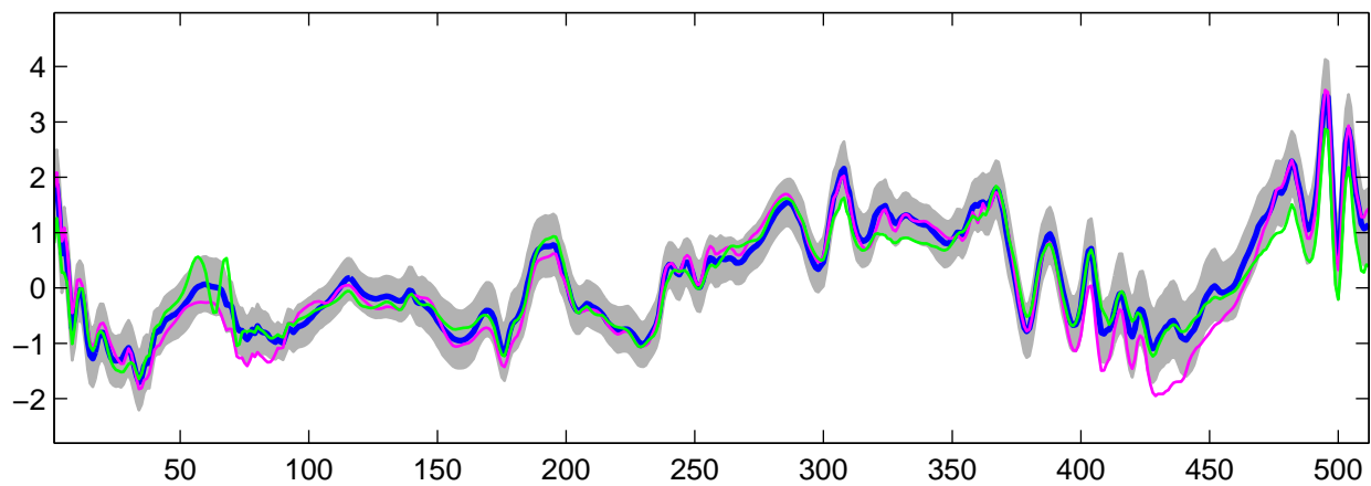
Estimated U_8(t) using R-WFMM: t_2 data, run 3
