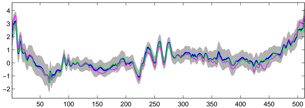
Estimated U_8(t) using G-WFMM: t_3 data, run 3
