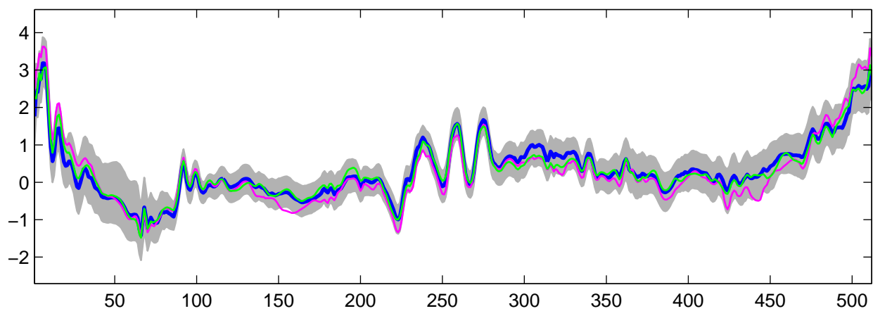
Estimated U_8(t) using R-WFMM: t_3 data, run 3
