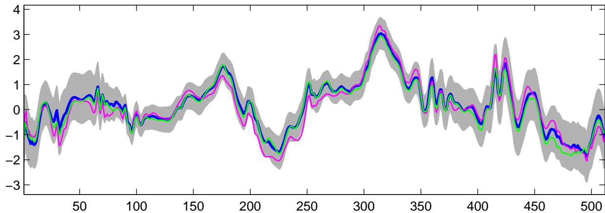
Estimated U_{\theta}(t) using G-WFMM: DE data, run 3
