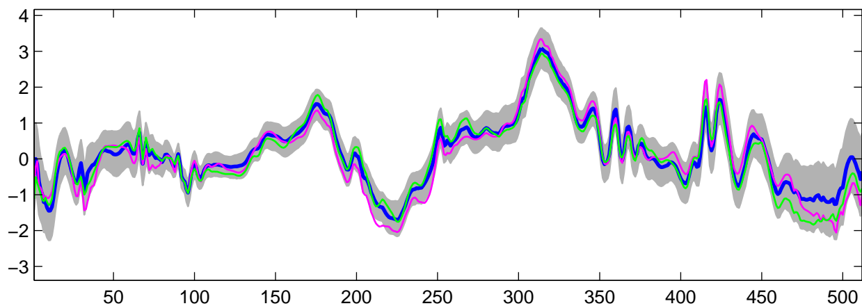
Estimated U_{\theta}(t) using R-WFMM: DE data, run 3
