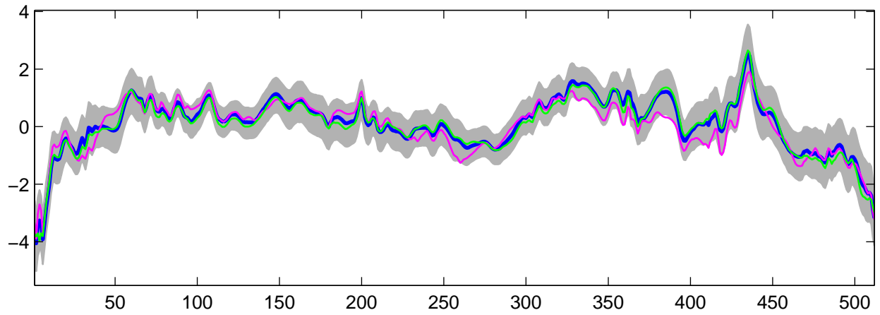
Estimated U_{\theta}(t) using G-WFMM: Normal data, run 3
