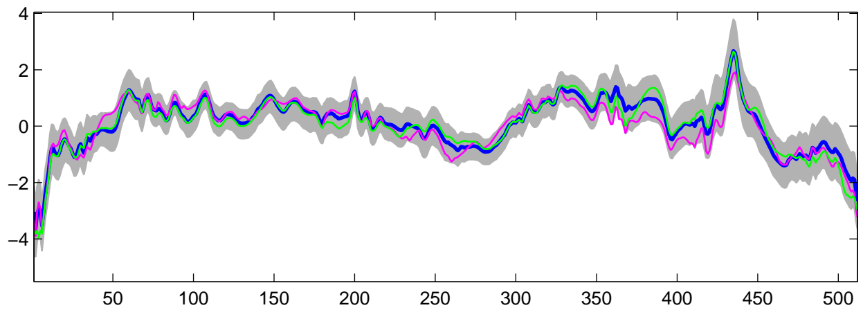
Estimated U_{\theta}(t) using R-WFMM: Normal data, run 3
