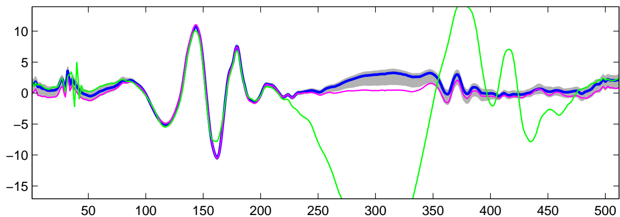
Estimated U_{\theta}(t) using R-WFMM: t_1 data, run 3
