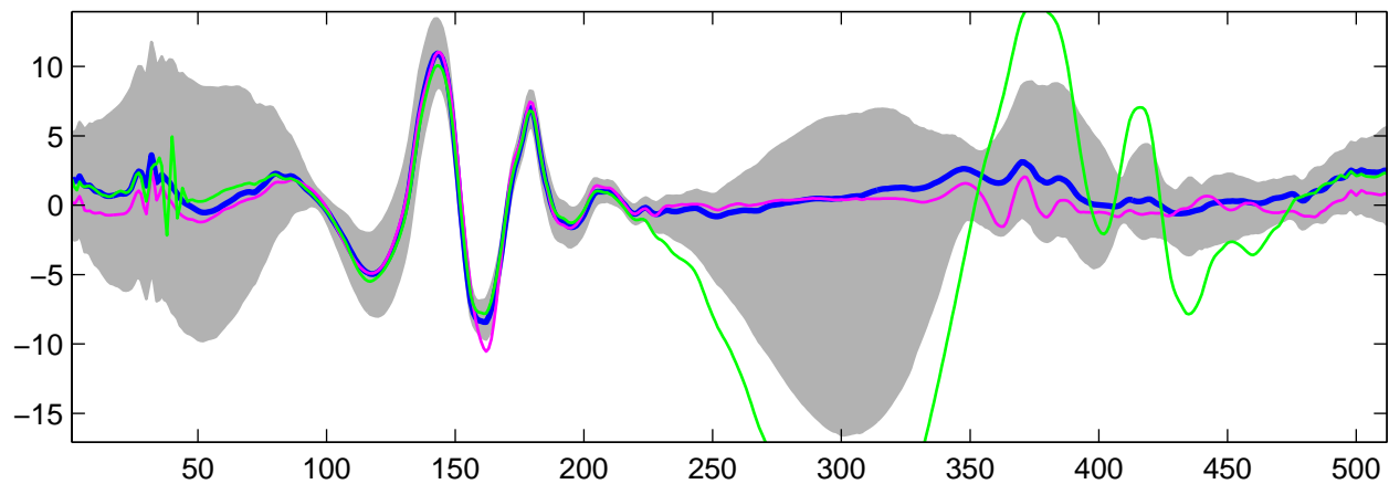
Estimated U_{\theta}(t) using G-WFMM: t_1 data, run 3
