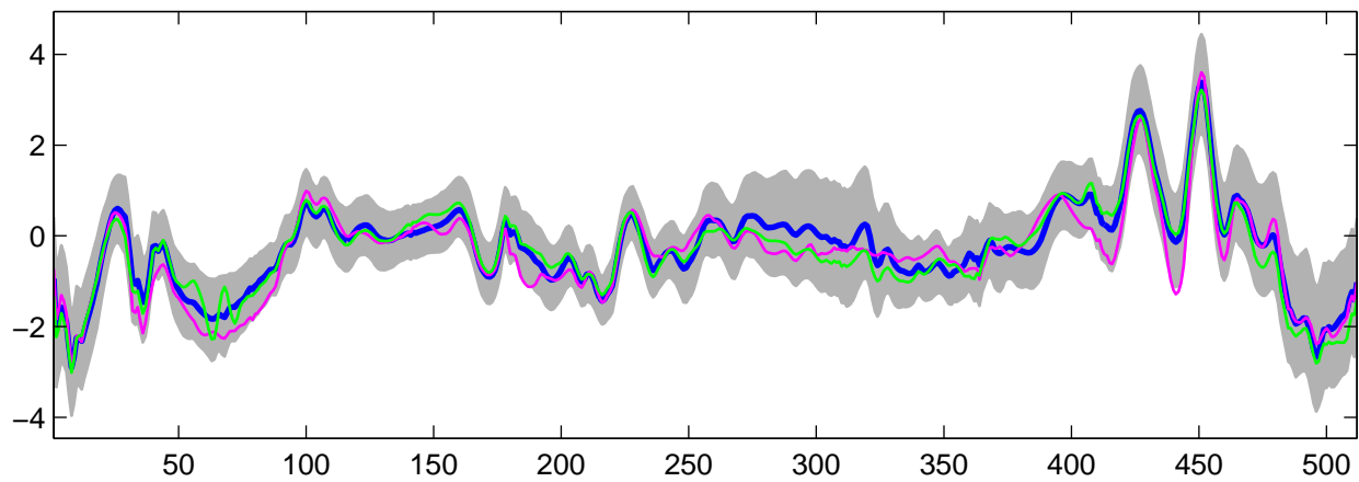
Estimated U_9(t) using G-WFMM: t_2 data, run 3
