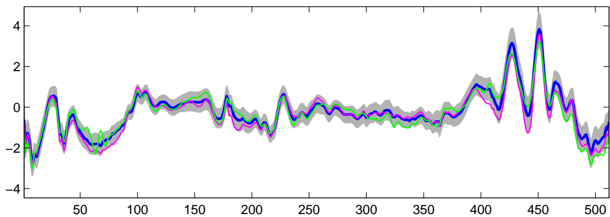
Estimated U_9(t) using R-WFMM: t_2 data, run 3
