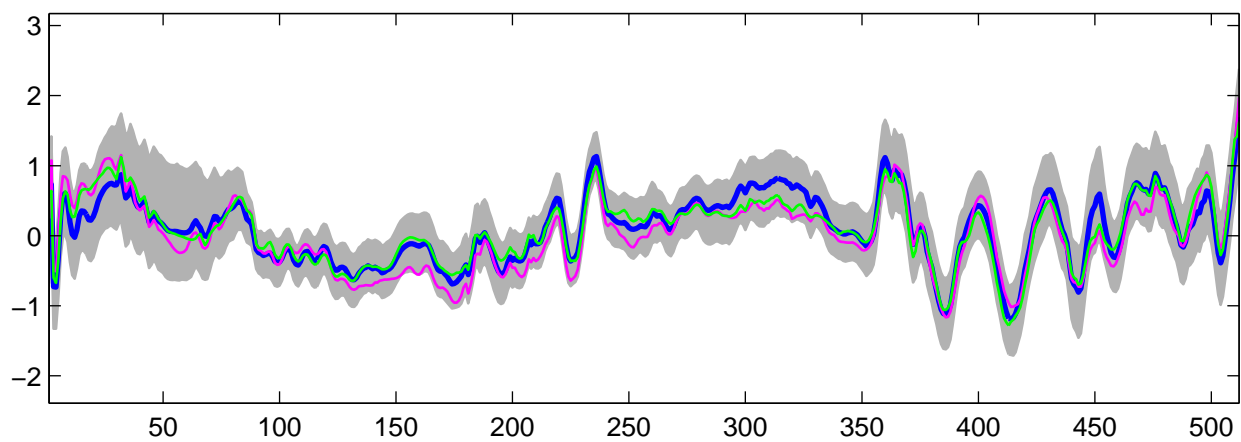
Estimated U_{\theta}(t) using R-WFMM: t_3 data, run 3
