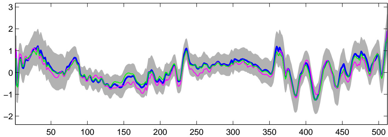
Estimated U_{\theta}(t) using G-WFMM: t_3 data, run 3
