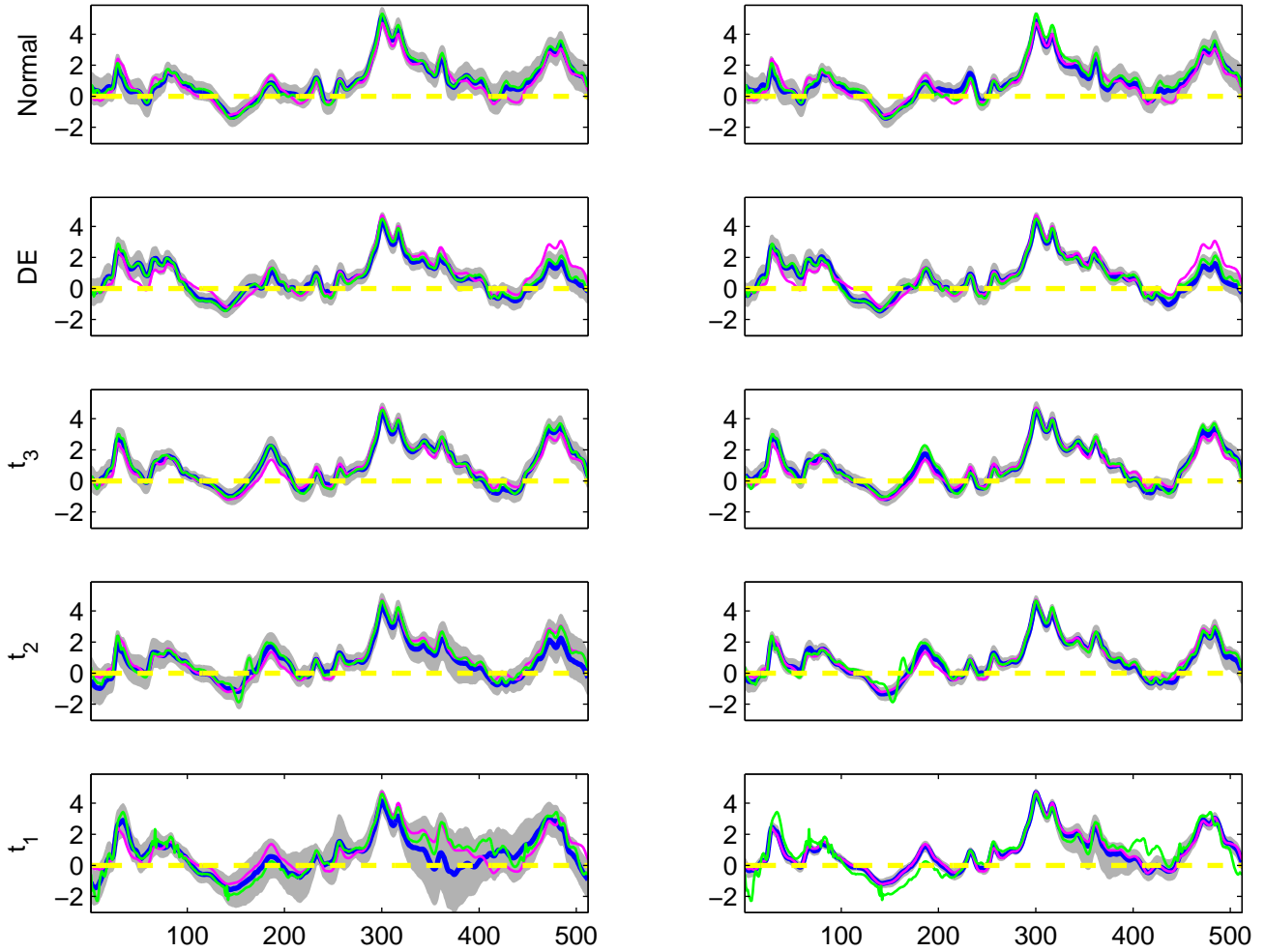
The estimated B_1(t) for 5 simulated datasets, simulation run 4 G-WFMM R-WFMM
