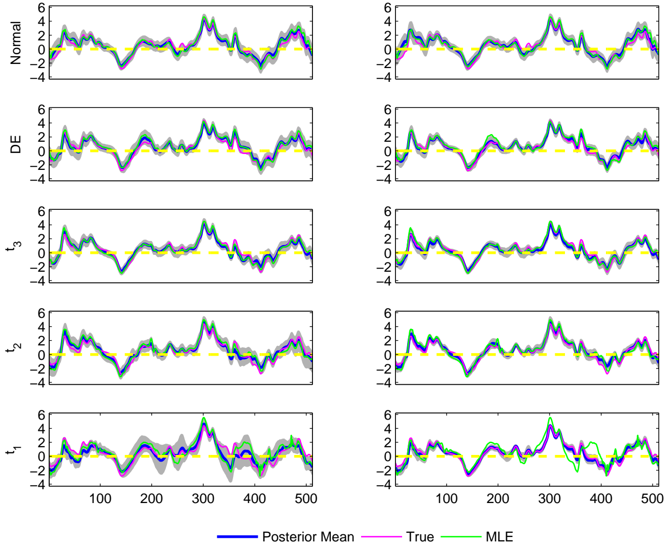
The estimated B_3(t) for 5 simulated datasets, simulation run 4
