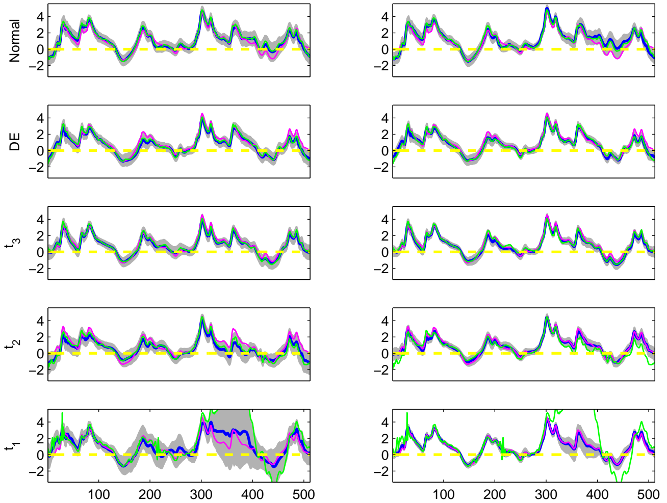
The estimated B_4(t) for 5 simulated datasets, simulation run 4
