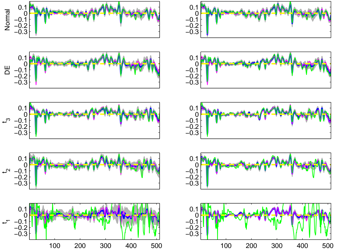
The estimated B_5(t) for 5 simulated datasets, simulation run 4 G-WFMM R-WFMM
