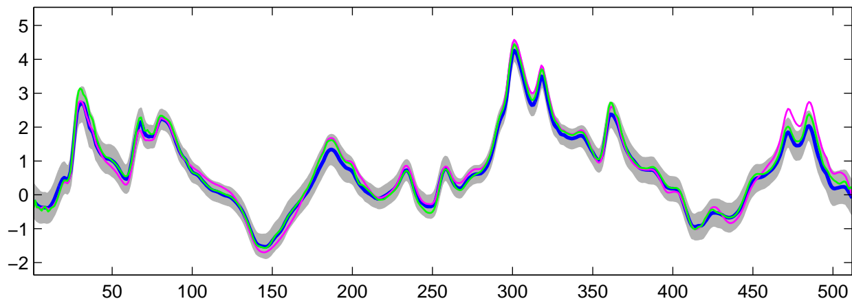
Estimated C_0(t) using G-WFMM: DE data, run 4
