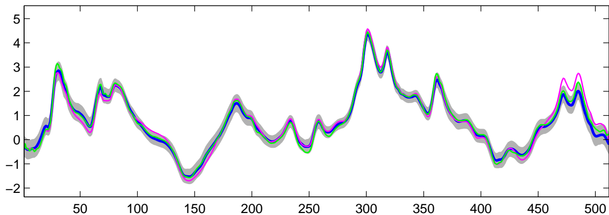
Estimated C_0(t) using R-WFMM: DE data, run 4
