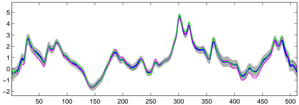
Estimated C_0(t) using R-WFMM: Normal data, run 4
