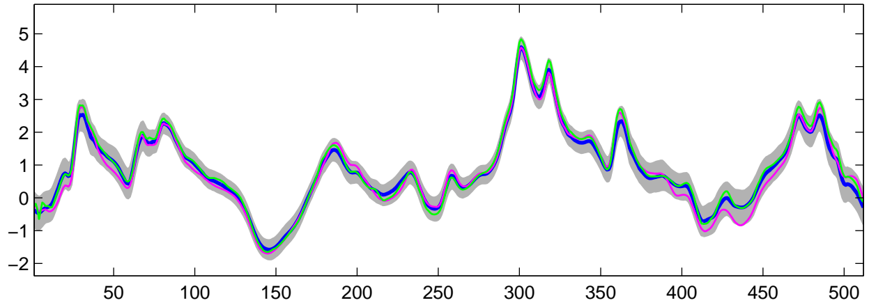
Estimated C_0(t) using G-WFMM: Normal data, run 4
