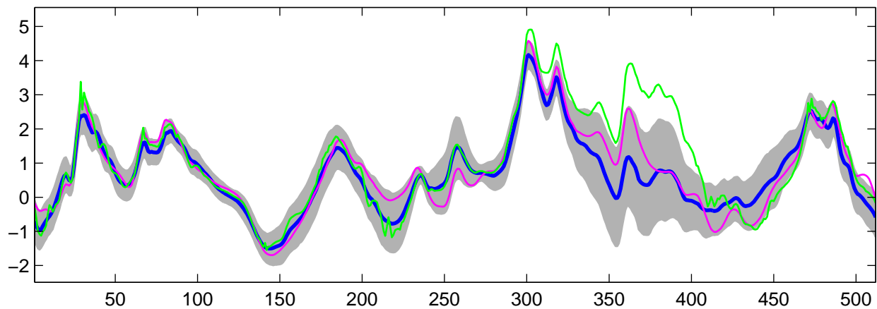
Estimated C_0(t) using G-WFMM: t_1 data, run 4
