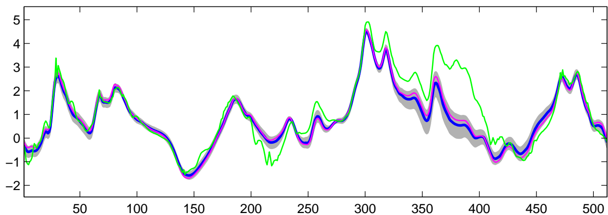
Estimated C_0(t) using R-WFMM: t_1 data, run 4
