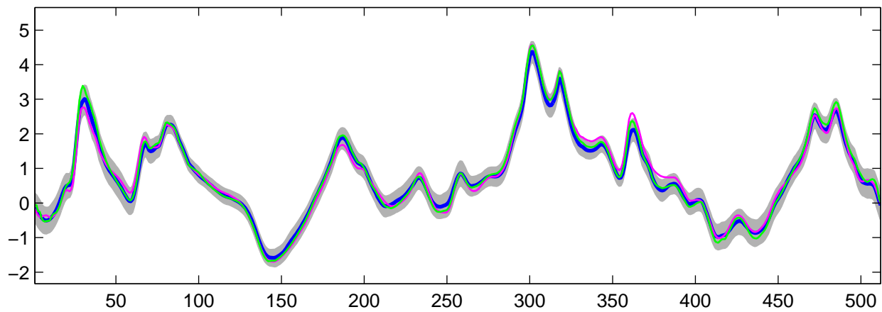
Estimated C_0(t) using G-WFMM: t_3 data, run 4
