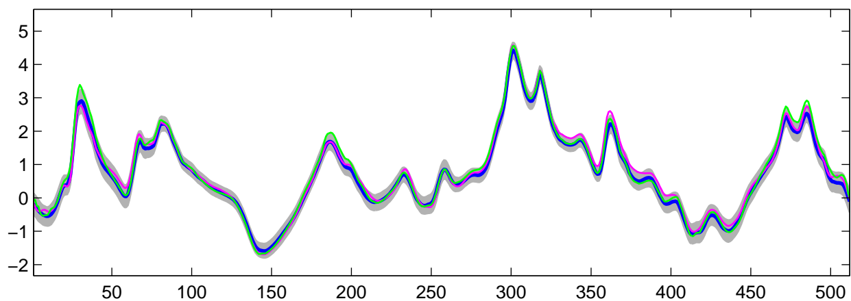
Estimated C_0(t) using R-WFMM: t_3 data, run 4
