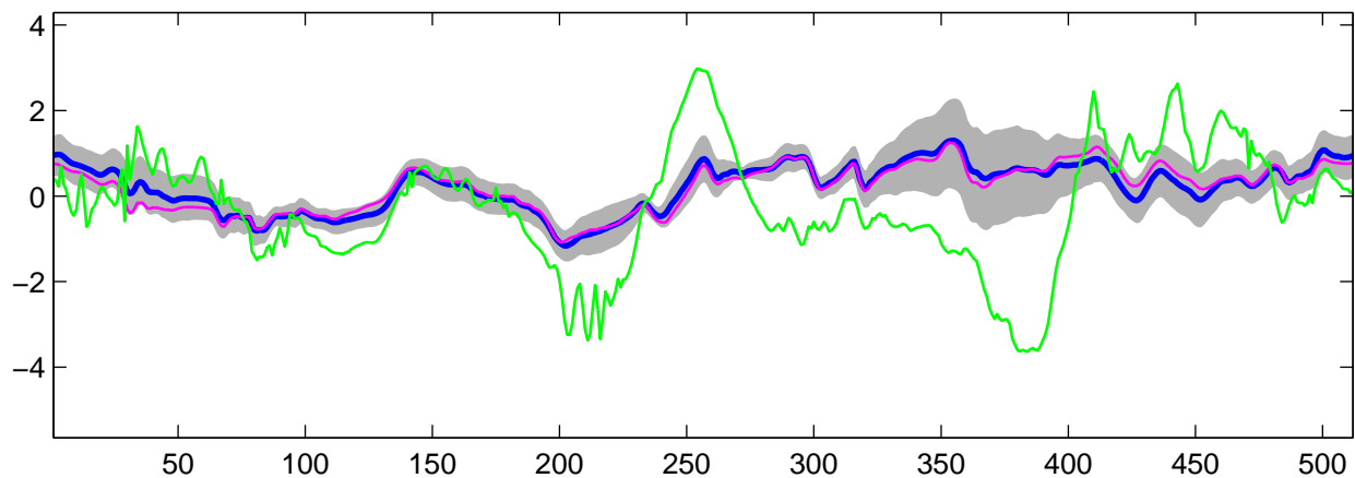
Estimated C_1(t) using R-WFMM: t_1 data, run 4
