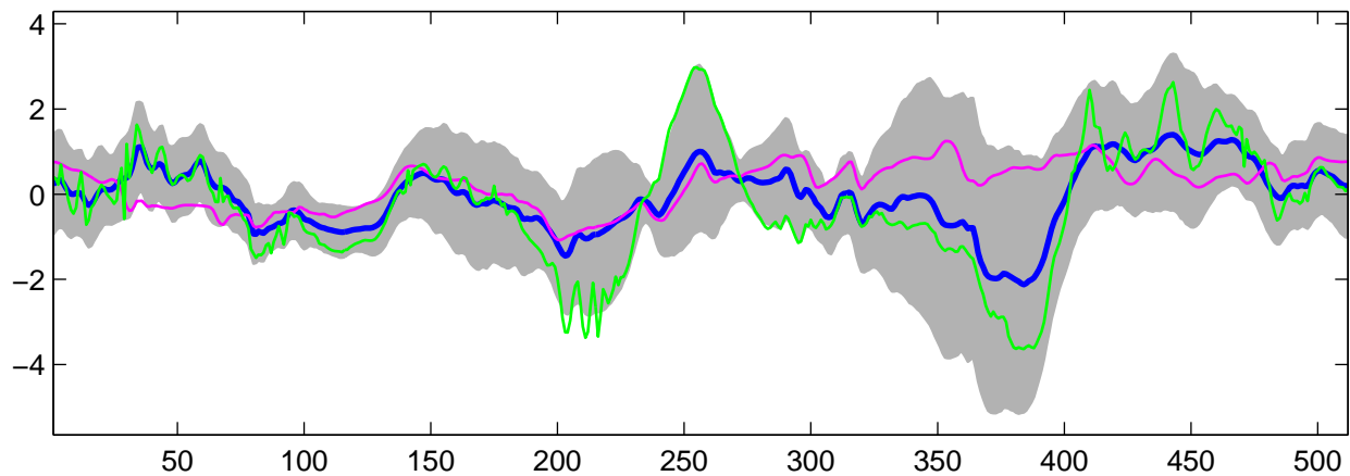
Estimated C_1(t) using G-WFMM: t_1 data, run 4
