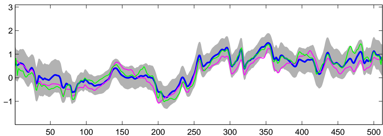
Estimated C_1(t) using R-WFMM: t_3 data, run 4
