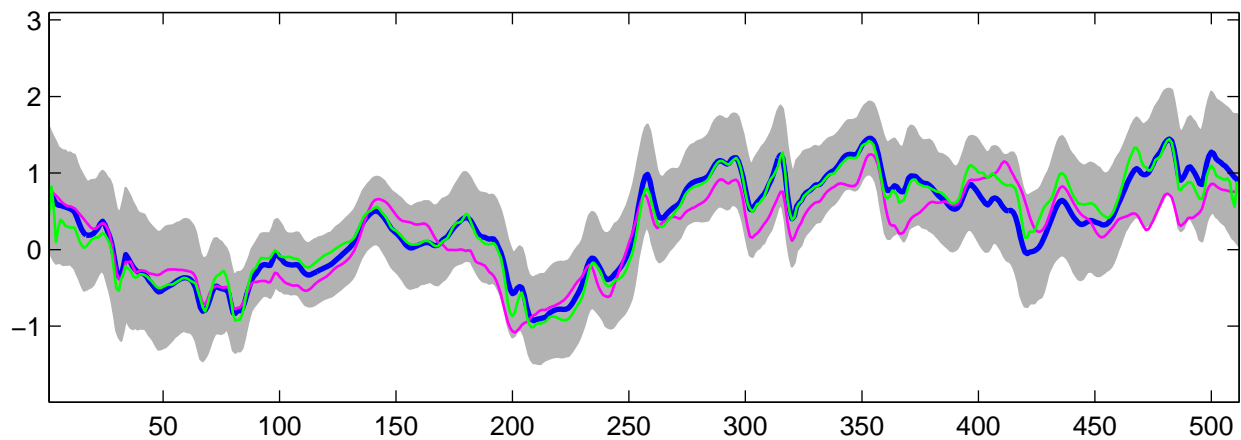
Estimated C_1(t) using G-WFMM: t_3 data, run 4
