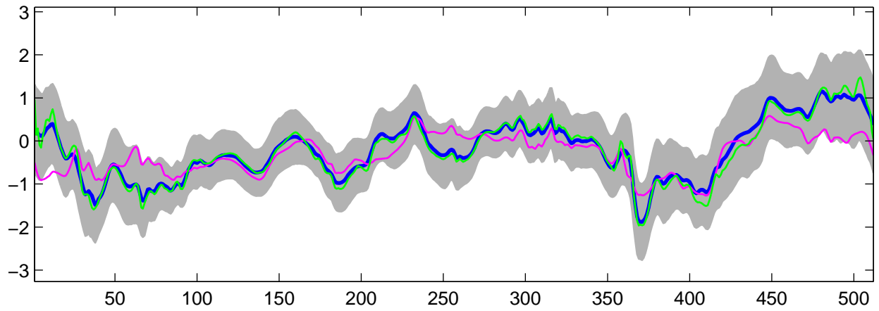
Estimated C_2(t) using G-WFMM: Normal data, run 4
