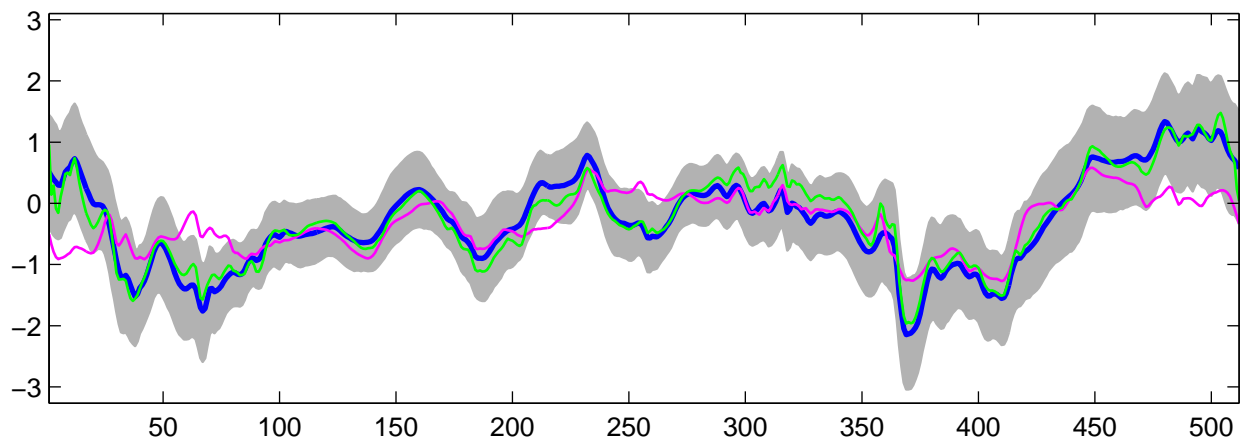
Estimated C_2(t) using R-WFMM: Normal data, run 4
