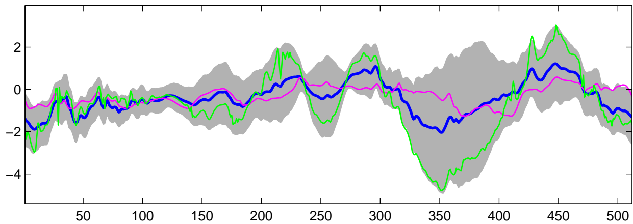
Estimated C_2(t) using G-WFMM: t_1 data, run 4
