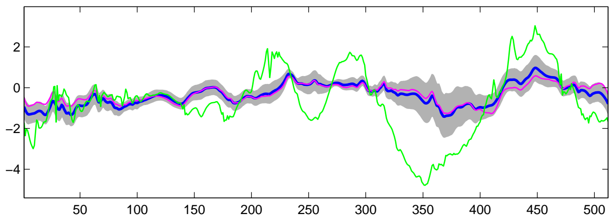
Estimated C_2(t) using R-WFMM: t_1 data, run 4
