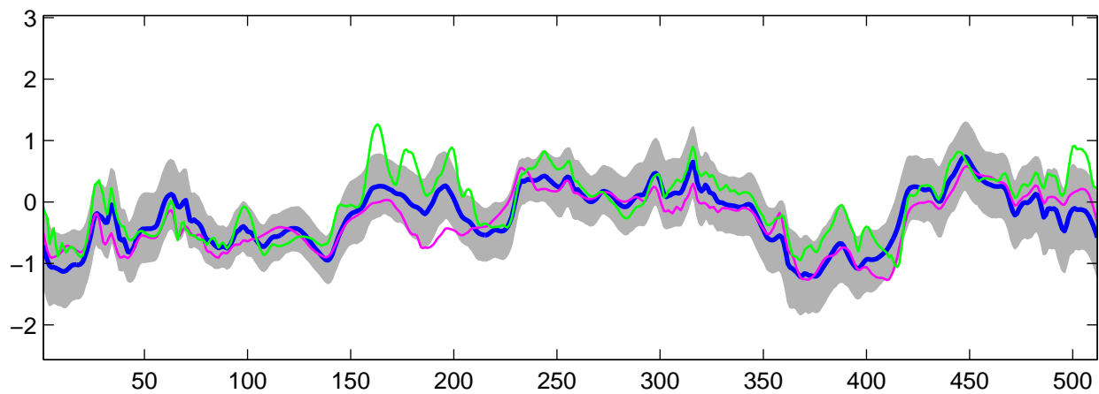
Estimated C_2(t) using R-WFMM: t_2 data, run 4
