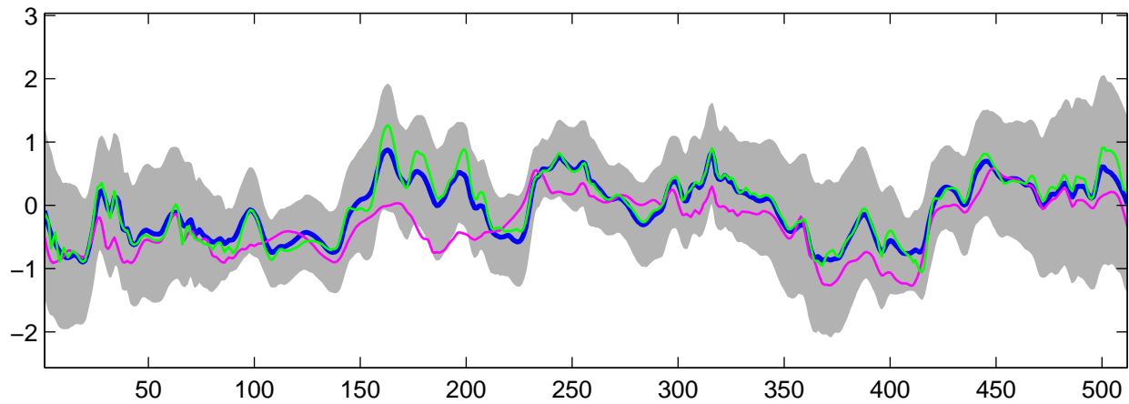
Estimated C_2(t) using G-WFMM: t_2 data, run 4
