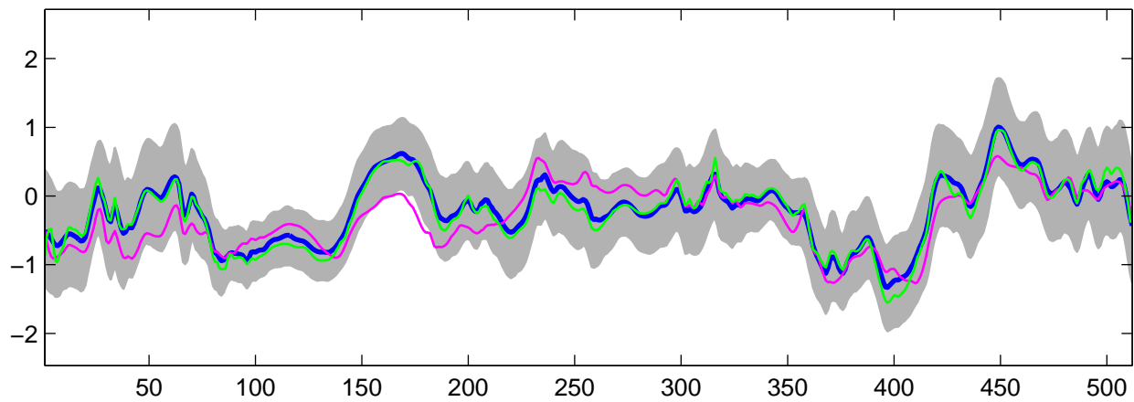
Estimated C_2(t) using G-WFMM: t_3 data, run 4
