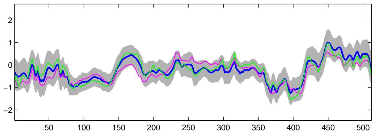
Estimated C_2(t) using R-WFMM: t_3 data, run 4
