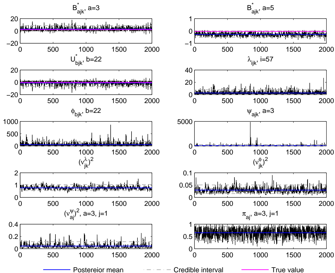
Trace plot, j=1, k=4 , DE data, simulation run 4
