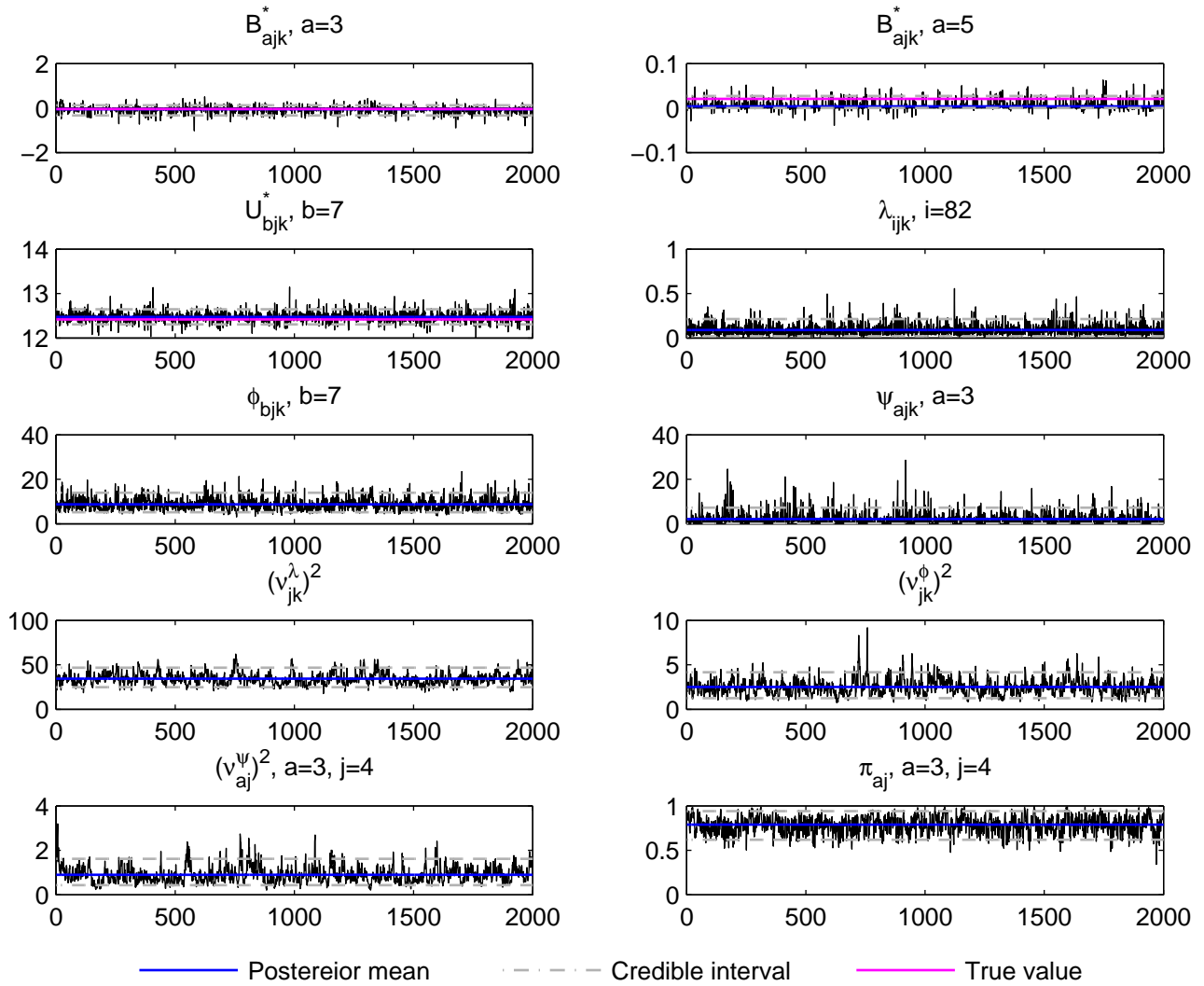
Trace plot, j=4, k=1, t_i data, simulation run 4
