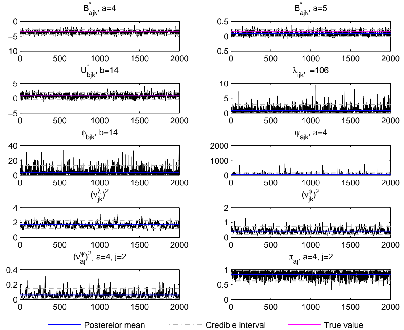
Trace plot, j=2, k=7, t_3 data, simulation run 4
