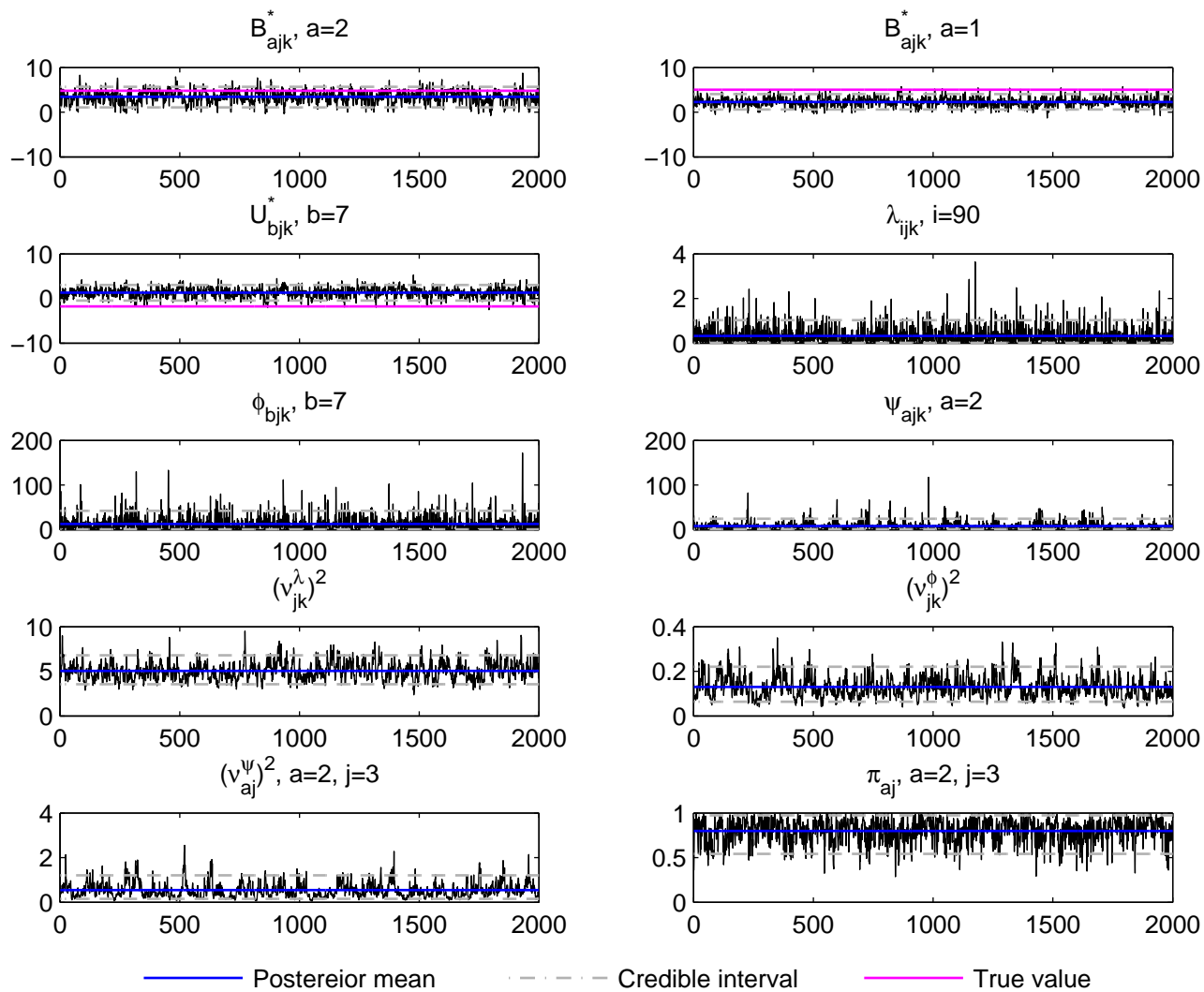
Trace plot, j=3, k=1 , Normal data, simulation run 4
