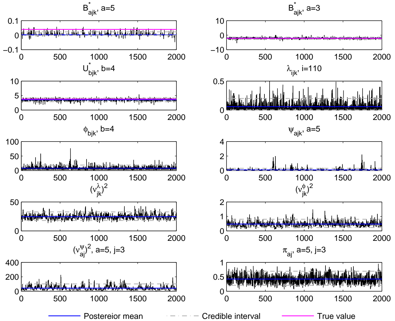
Trace plot, j=3, k=3, t_j data, simulation run 4
