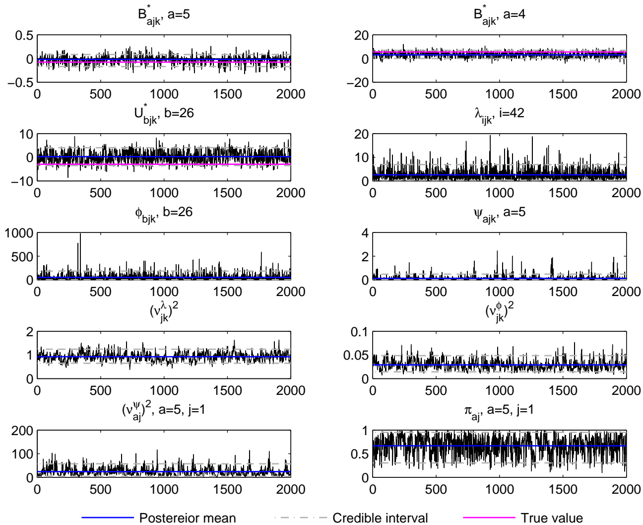
Trace plot, j=1, k=7 , DE data, simulation run 4
