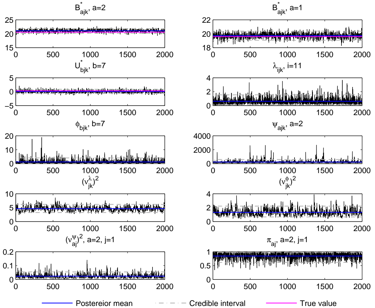
Trace plot, j=1, k=1, t_i data, simulation run 4
