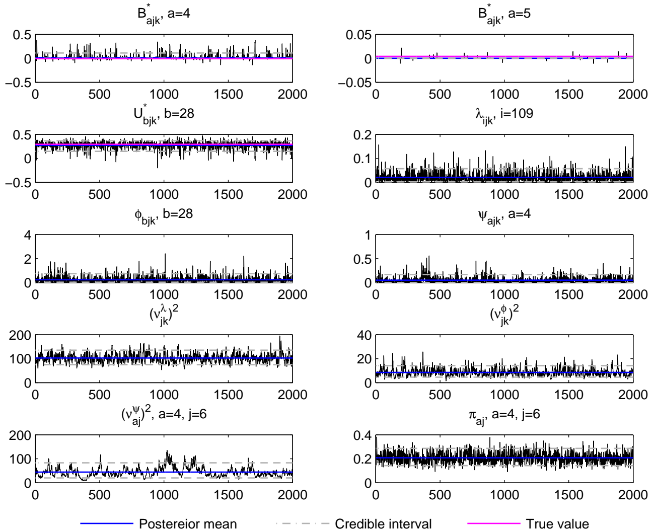
Trace plot, j=6, k=1, t_2 data, simulation run 4
