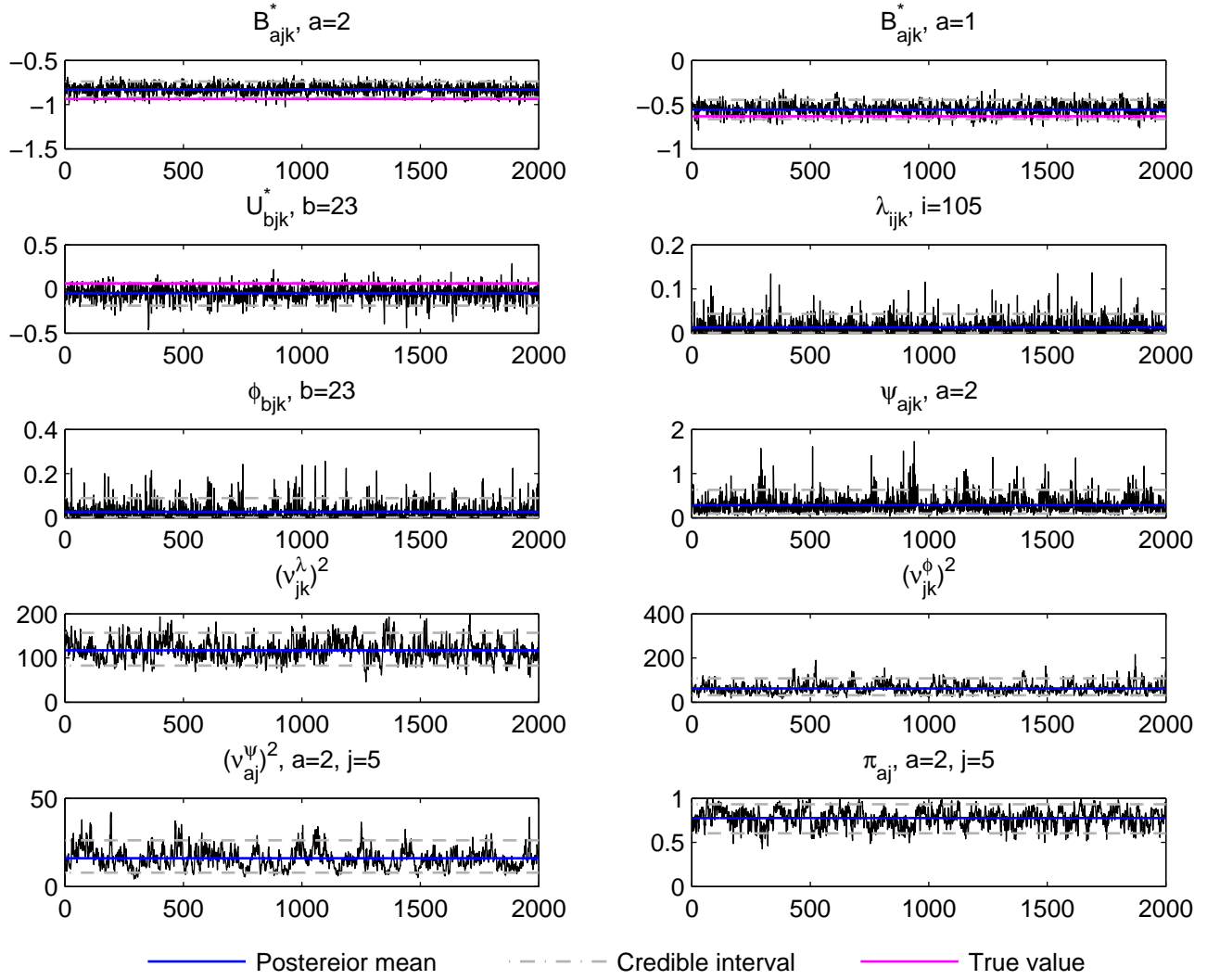
Trace plot, j=5, k=4, t_3 data, simulation run 4
