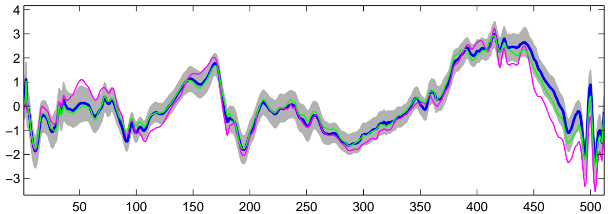
Estimated U_{10}(t) using R-WFMM: DE data, run 4
