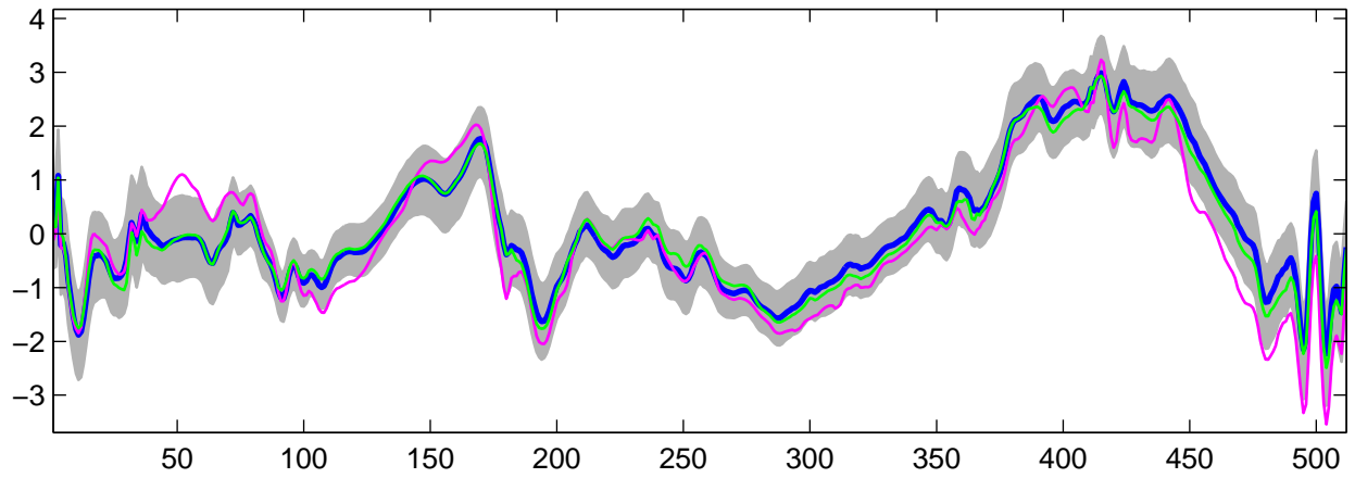
Estimated U_{10}(t) using G-WFMM: DE data, run 4
