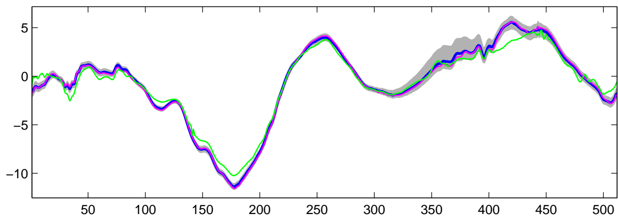
Estimated U_{10}(t) using R-WFMM: t_1 data, run 4
