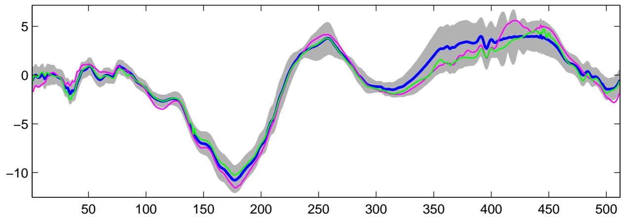
Estimated U_{10}(t) using G-WFMM: t_1 data, run 4
