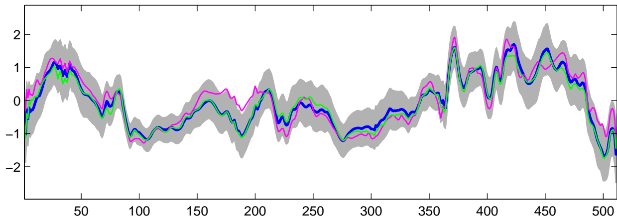
Estimated U_{10}(t) using G-WFMM: t_3 data, run 4
