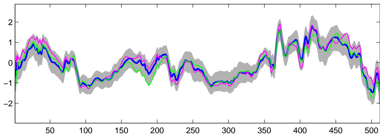
Estimated U_{10}(t) using R-WFMM: t_3 data, run 4
