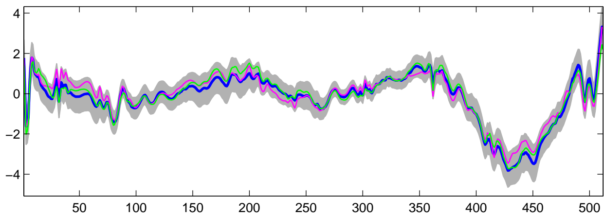
Estimated U_{11}(t) using R-WFMM: DE data, run 4
