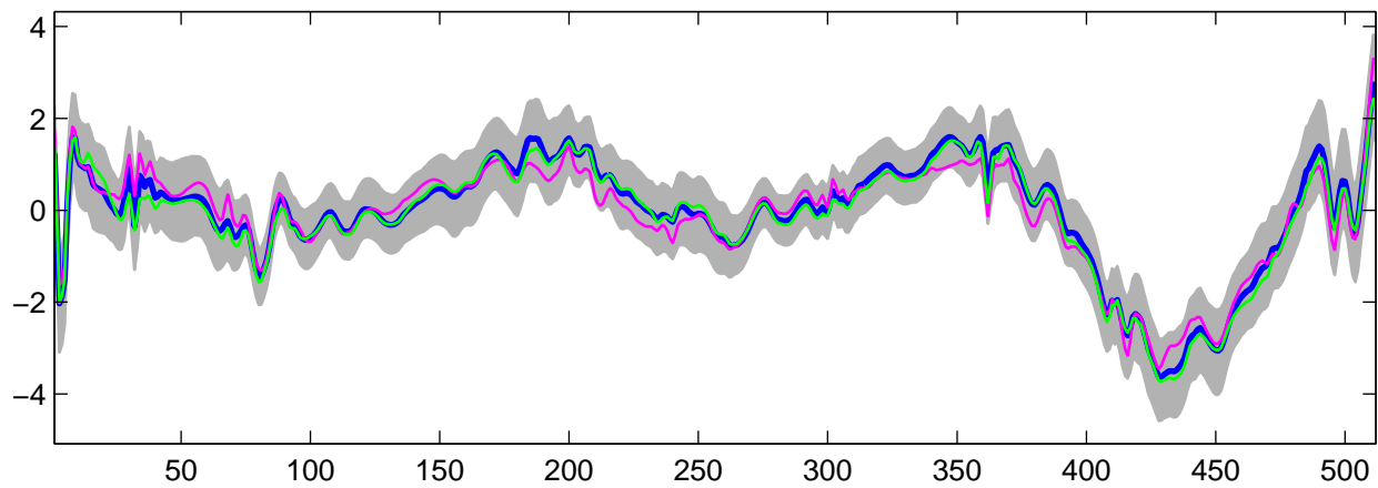
Estimated U_{11}(t) using G-WFMM: DE data, run 4
