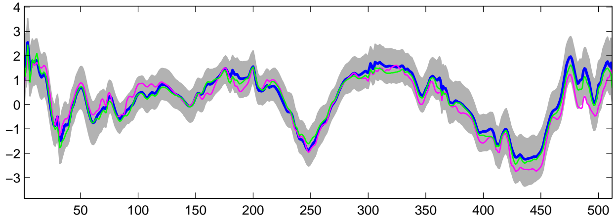
Estimated U_{11}(t) using G-WFMM: Normal data, run 4
