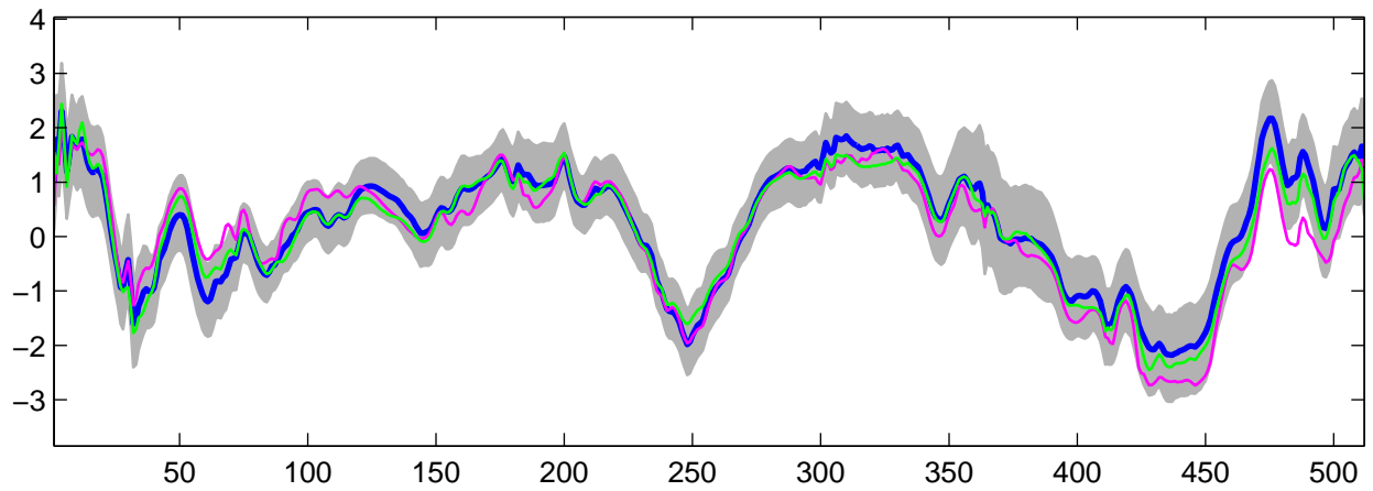
Estimated U_{11}(t) using R-WFMM: Normal data, run 4
